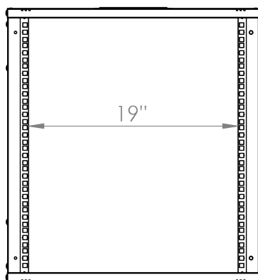
Front inside view
