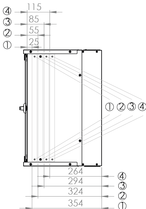
19" cabinet in the top view
